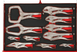
TTEVG11 11 piece power grip plier set
