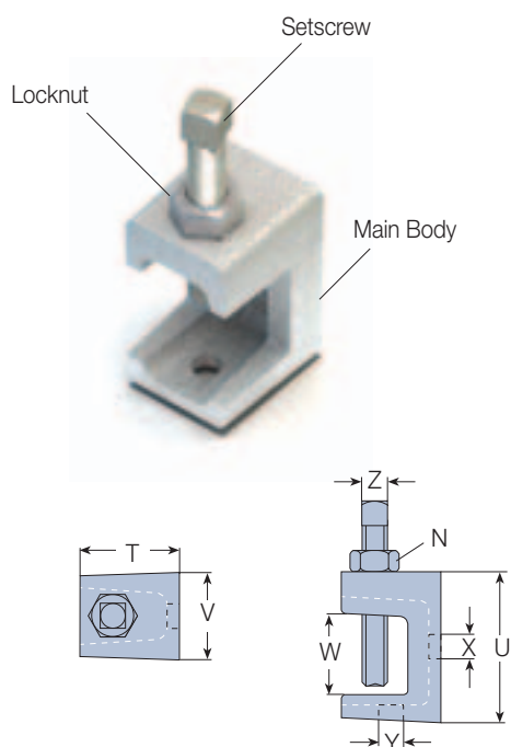
Beam clamp with tapped holes in position X and Y to accept threaded rod or cable clips. For parallel or tapered flanges. Supplied with grade 8.8 cup point setscrew.
