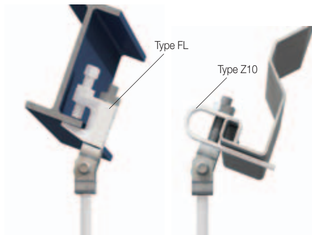
Swivel unit for applications on inclined beams. Can be used with type FL or type Z10. Supplied complete with grade 8.8 M10 x 90 setscrew and nut.
